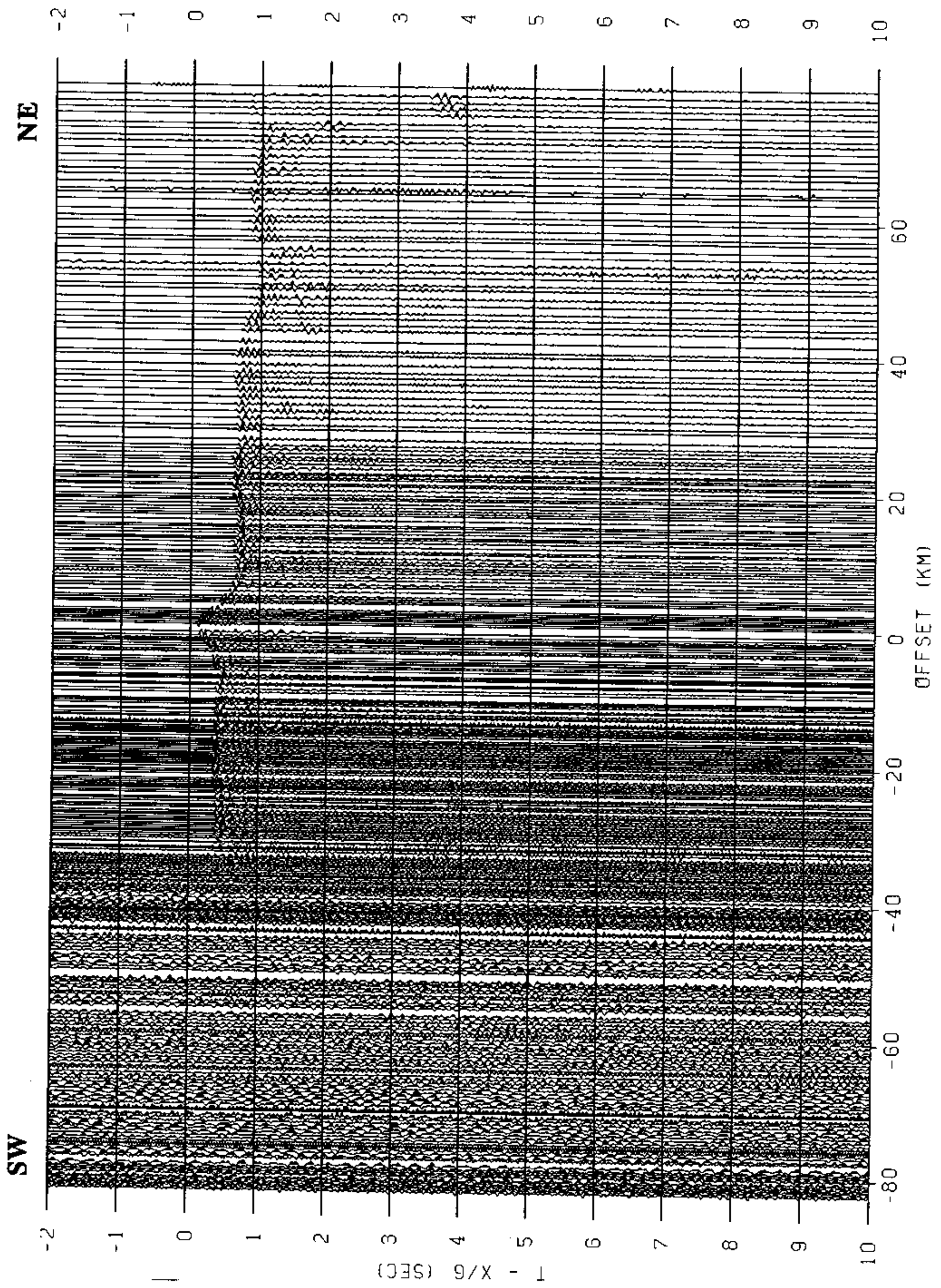
Figure 60. Shot 53 Shotpoint 8351
