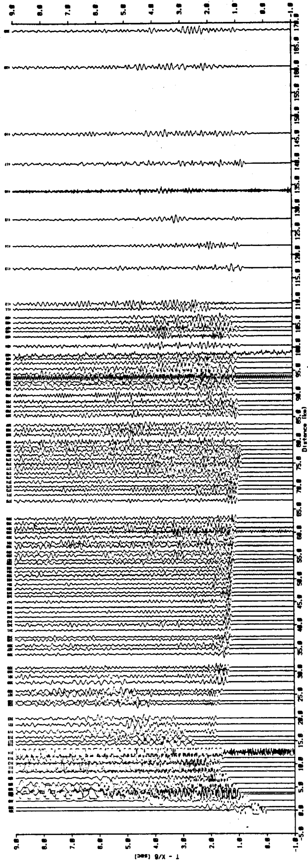
Shot 11, Shotpoint 24
