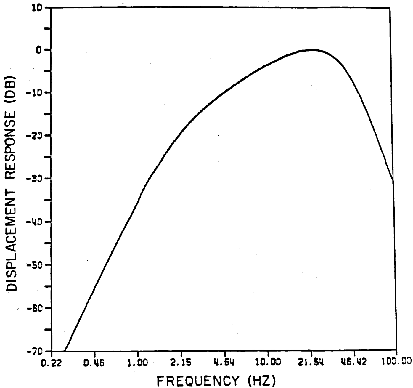
Figure 18: System response curve for cassette recording units with 2-Hz seismometers
