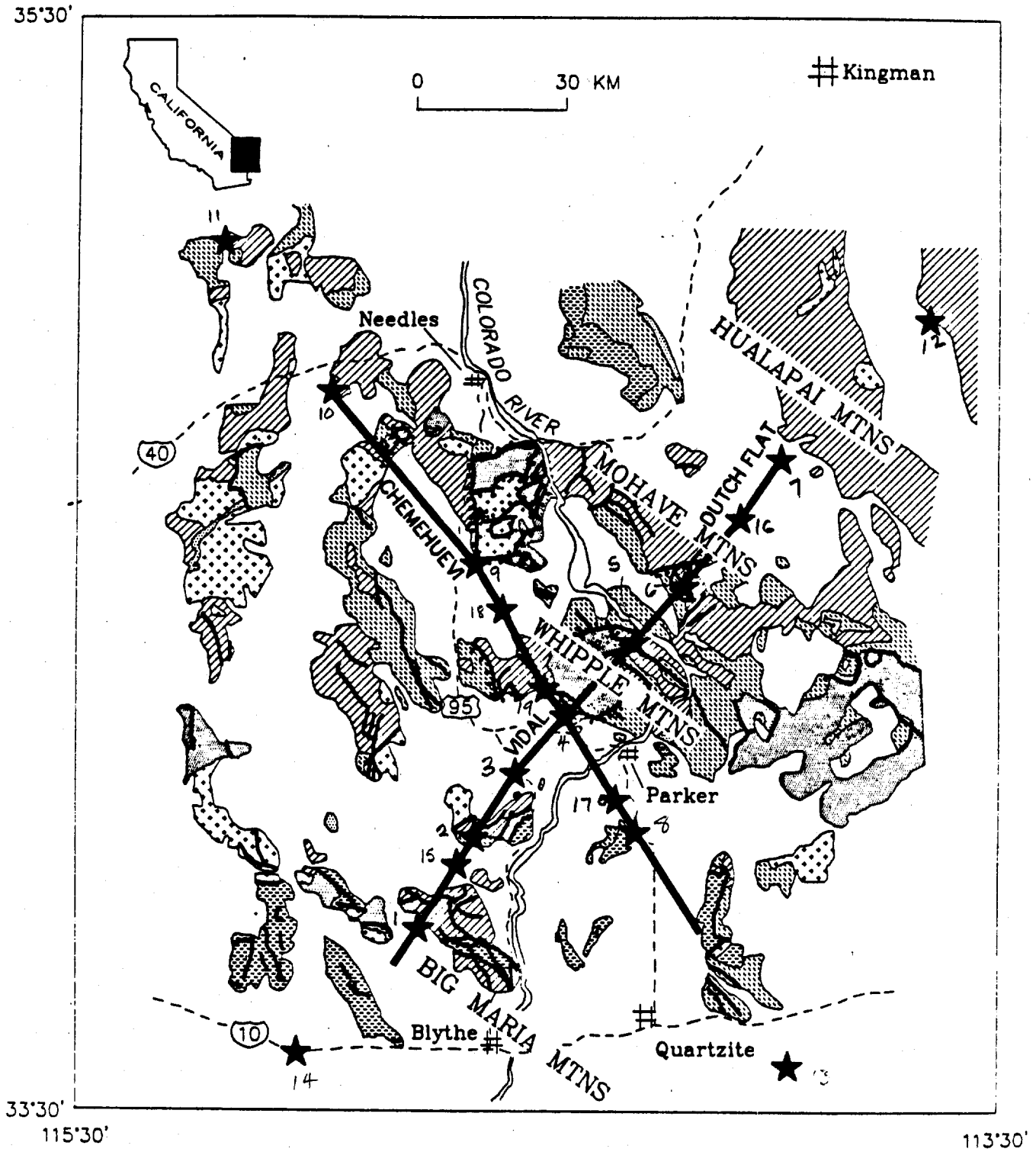
Figure 1: Geologic Map of Study Area, Compiled from Howard (1986), Jennings (1977), Reynolds (1980), and Wilson (1969).
