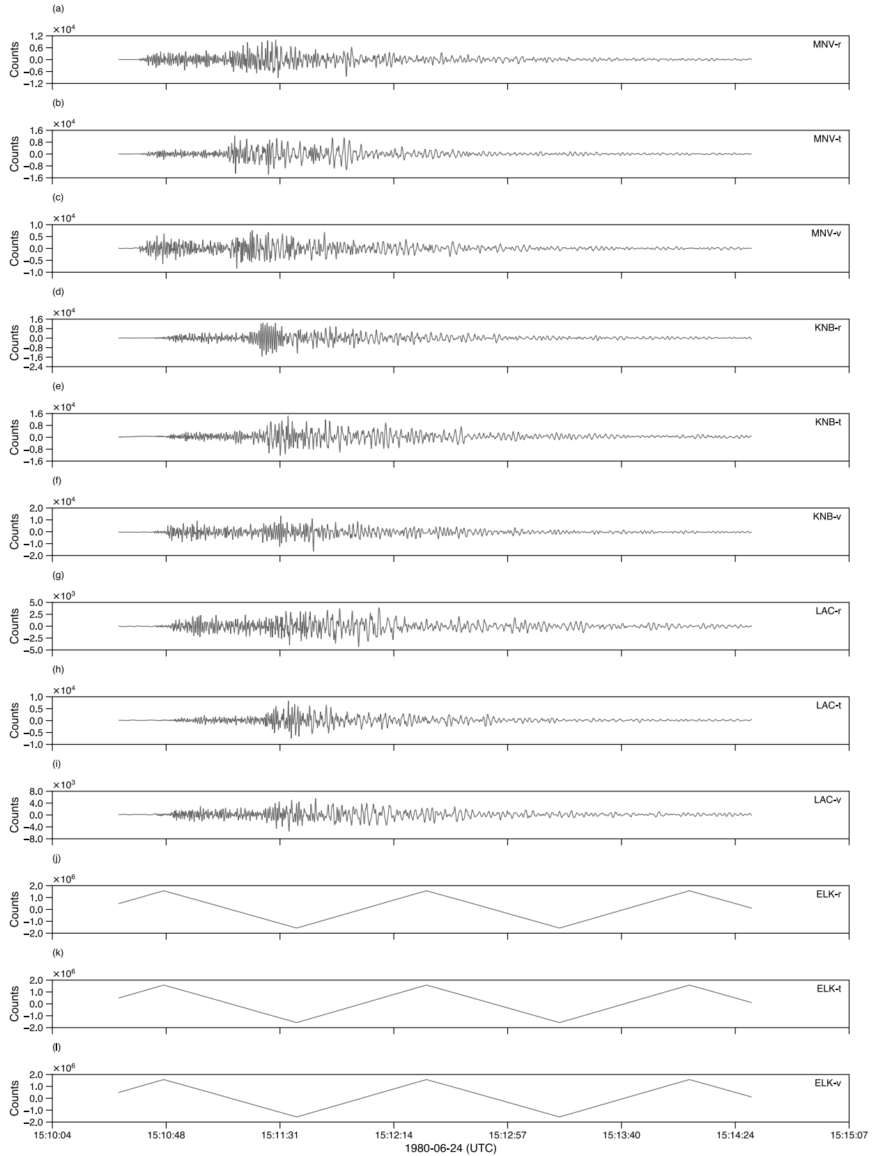
Figure 4: LNN waveform recordings of event 21 with an identified QC issue. ELK recordings are non-seismic triangular-wave recordings.
