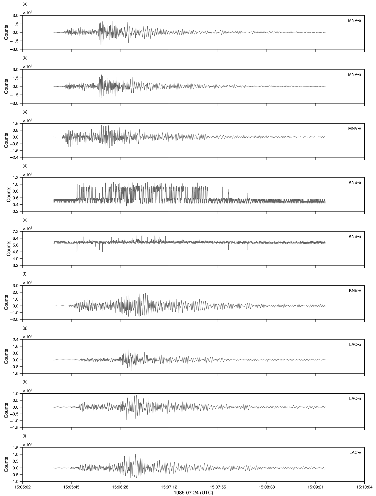
Figure 6: LNN waveform recordings of event 98 with an identified QC issue. KNB e - and n - component waveforms have noise characteristic of sensor and/or cable issues, such as corrosion.
