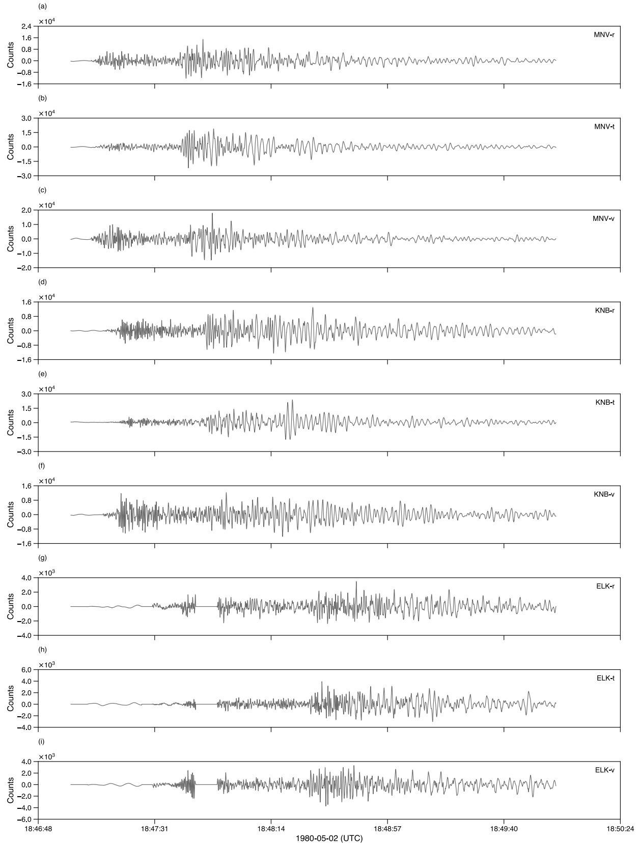
Figure 8: LNN waveform recordings of event 18 with an identified QC issue. All ELK waveforms have a gaps for ~8 seconds 15 seconds after the P-wave arrival.
