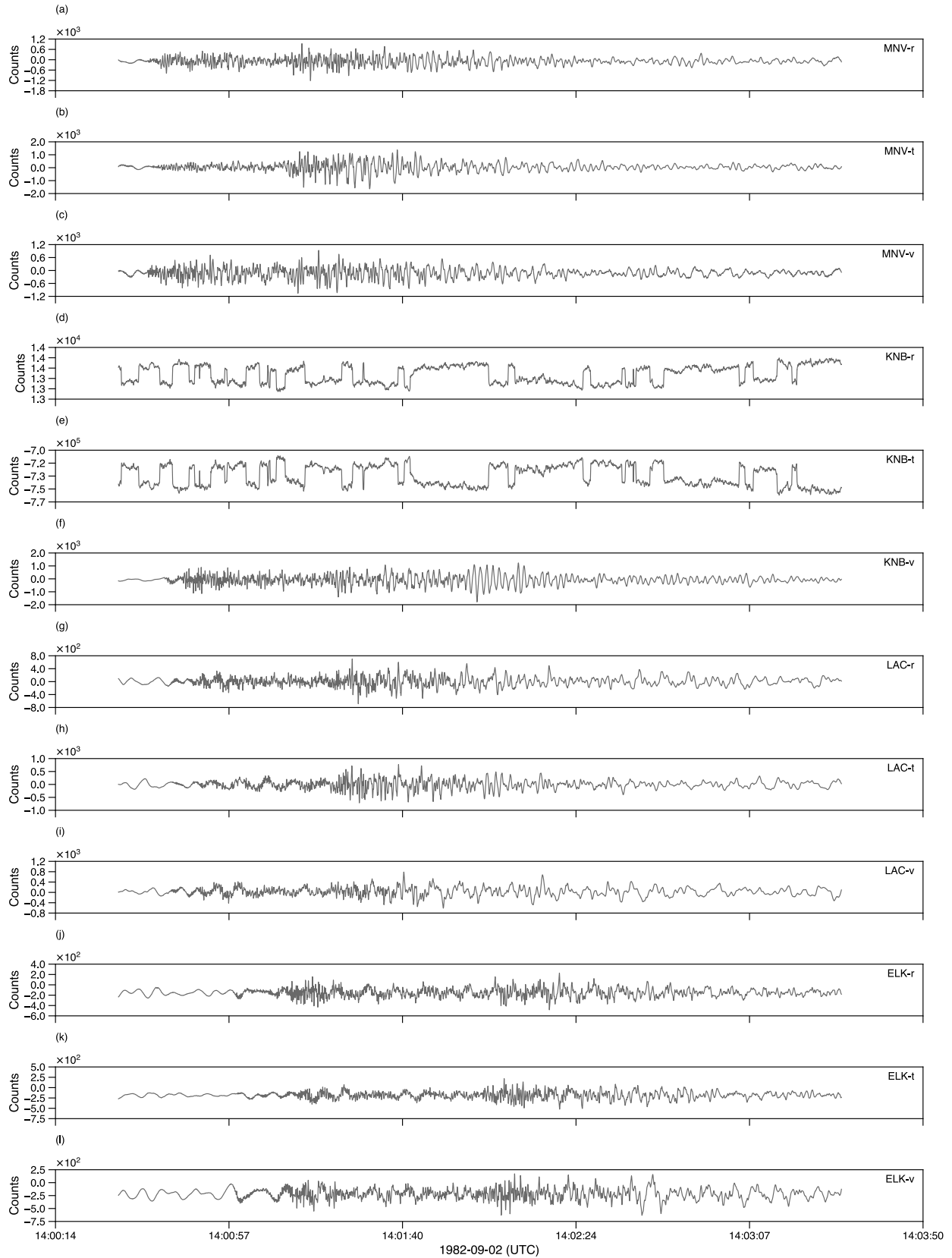
Figure 5: LNN waveform recordings of event 53 with an identified QC issue. KNB r- and t- component waveforms have noise characteristic of sensor and/or cable issues, such as corrosion.
