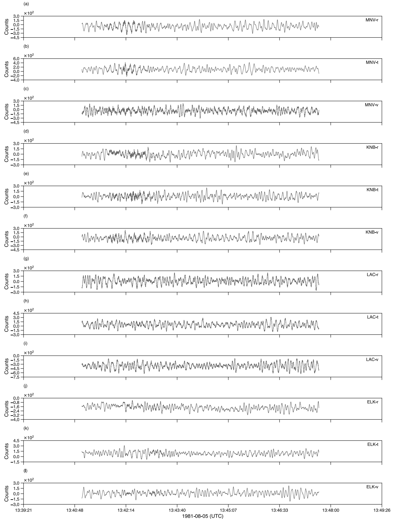
Figure 7: LNN waveform recordings of event 35 with an identified QC issue. All station's waveforms have low SNR and filtering will enhance the SNR.
