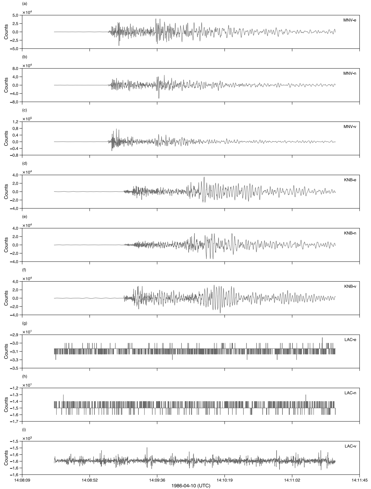
Figure 3: LNN waveform recordings of event 93 with an identified QC issue. LAC recordings are non-seismic noise recordings and e- and n- channels are digitizer noise.
