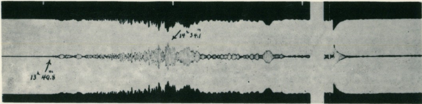
BOMBAY, INDIA. Milne Seismograph. ( From photographic copy. )
