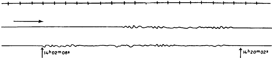
CALAMATE, GREECE. Agamennone Vertical Pendulum. ( From hand-tracing. )
