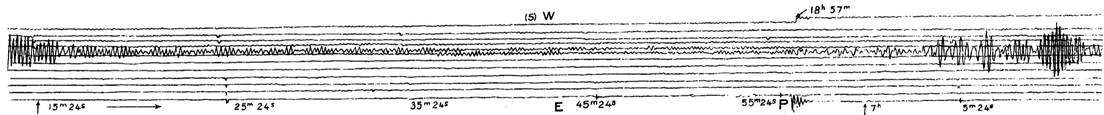
GRANDE SENTINELLA, ISCHIA, ITALY. Grablowitz Horizontal Pendulum. ( From photographic copy. )
