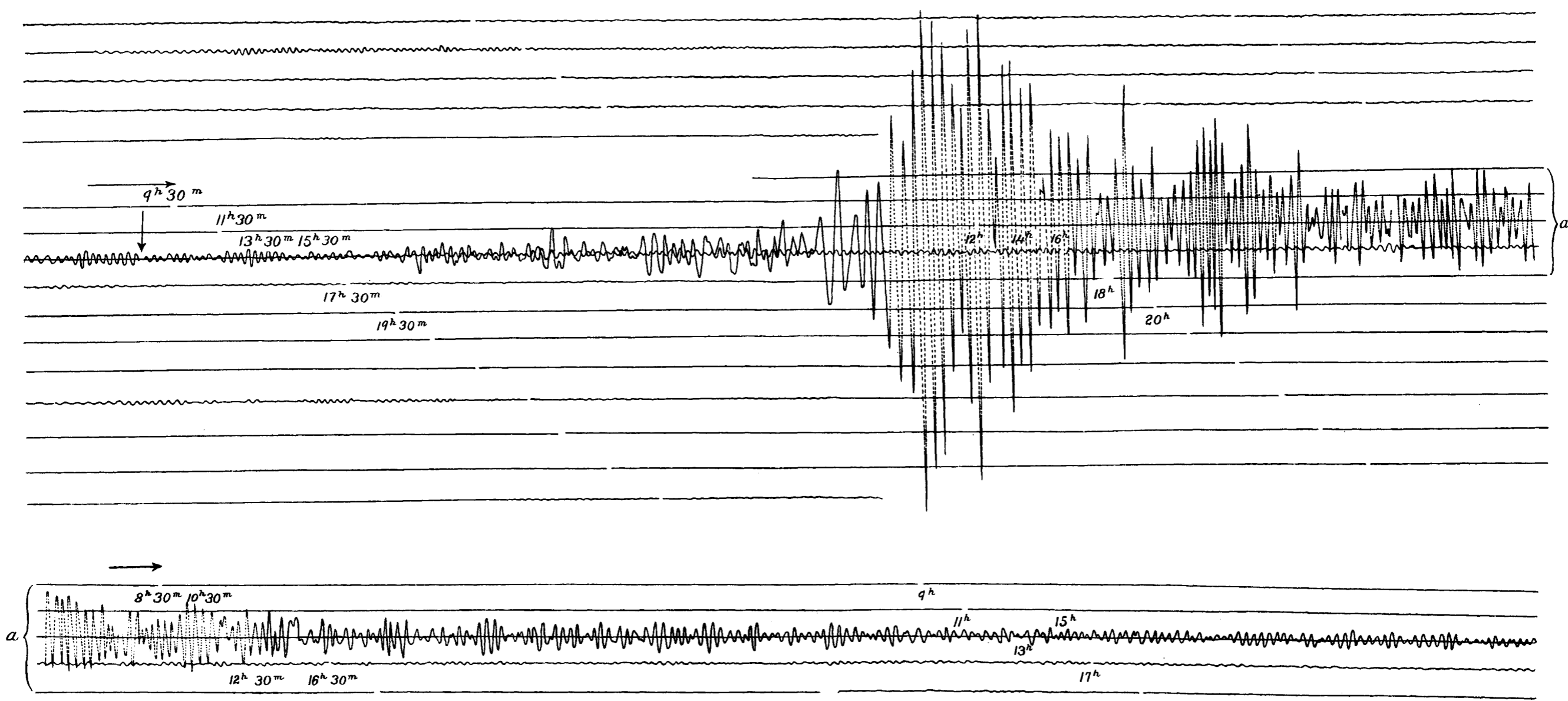
POTSDAM, GERMANY. Von Rebeur-Paschwitz Horizontal Pendulum. Modified by Dr. Hecker, E-W component. (From photographic copy.) Correction to G. M. T. from beginning of time-breaks, -20 s .
