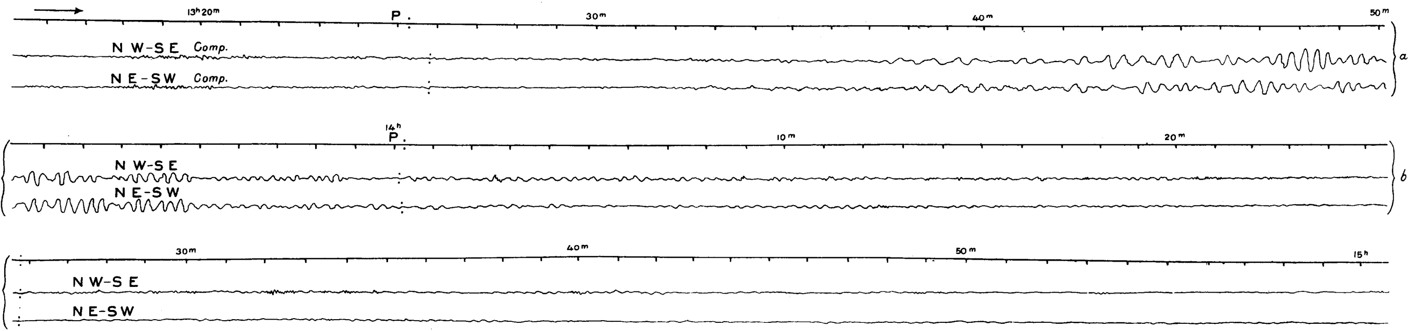
ROCCA DI PAPA, ITALY. Agamennone Microseismometrograph, 500 Kilos. (From hand-tracing.) Correction to G. M. T.=+18 m 49 s .
