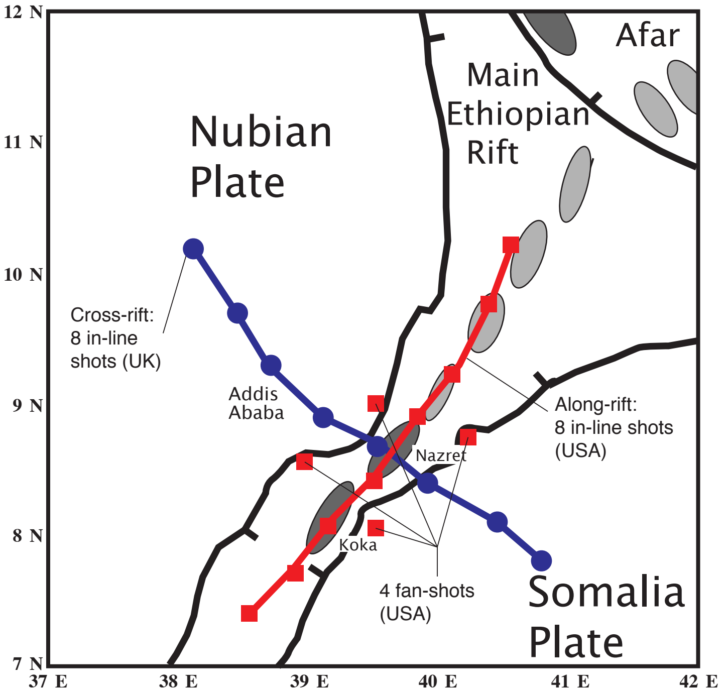
Figure 9. Proposed CD seismic experiment.
